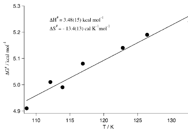
Figure 4. Gibbs free energies of activation ( \Delta G^\ddagger ) for equatorial to axial conformational inversion of 8 . Corresponding average \Delta H^\ddagger and \Delta S^\ddagger values for the temperature range (110–130 K) are derived from the expression \Delta G^\ddagger = \Delta H^\ddagger - T\Delta S^\ddagger .
