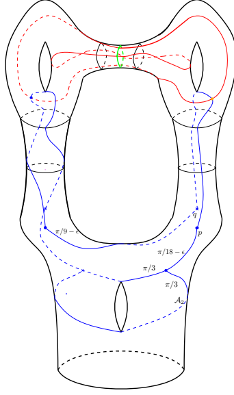
Figure 11.6. The final mixed tête-à-tête graph (\Gamma^\bullet, \delta_\bullet) . In green we have \Gamma^2 ; in red we have \Gamma^1 \setminus \Gamma^2 and in blue \Gamma \setminus \Gamma^1 .
