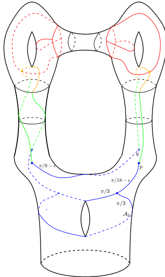
Figure 11.5. The relative tête-à-tête graph (\Gamma[1], \mathcal{B}[1]) embedded in \Sigma^1 \subset \Sigma . The lengths are indicated. The green lines correspond to retraction lines of the corresponding product structures \eta_1 and \eta_2 and the orange lines correspond to retraction lines of the product structures chosen for the cylinders \Sigma^2_{\Gamma[1]^1} .
