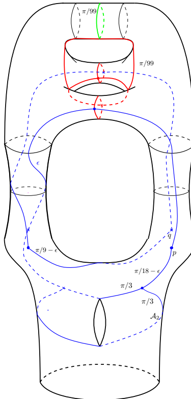
Figure 11.9. The final mixed tête-à-tête graph \Gamma . Each red edge has length \pi/99 , the green circle also has length \pi/99 , the for blue edges that go from \Sigma^0 to \Sigma^1 have length \epsilon . The rest of the edges is the same as in the previous example.
