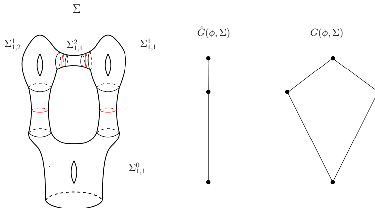
Figure 11.2. On the left we see the surface \Sigma . On the right we see the corresponding graphs \hat{G}(\phi, \Sigma) and G(\phi, \Sigma) for the depicted almost-canonical form. In red we see the core curves of the annuli in \mathcal{A} .
