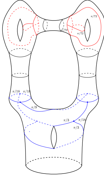
Figure 11.3. The relative tête-à-tête graph (\Gamma[0], \mathcal{B}[0]) embedded in \Sigma^0 \subset \Sigma . The lengths are indicated on a few edges and the rest is obtained by symmetry of the graph. We can also see in red an invariant relative spine for \Sigma^1 .
