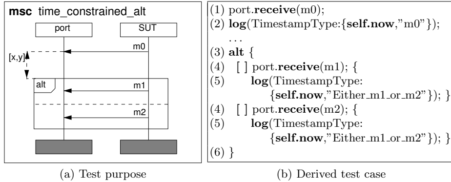
Fig. 6. Time constrained observation attached to first event of alternative
