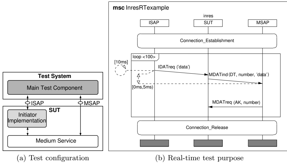
Fig. 2. Test architecture and test purpose for the Inres test case example
