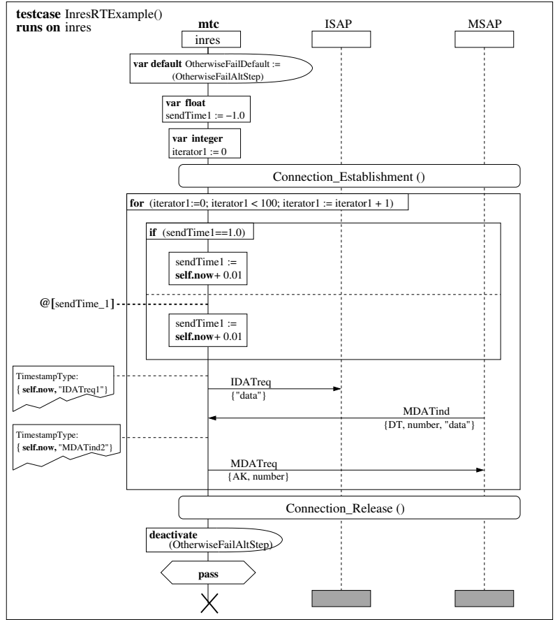
Fig. 8. TIMEDGFT presentation of the Inres test case in Fig. 3
