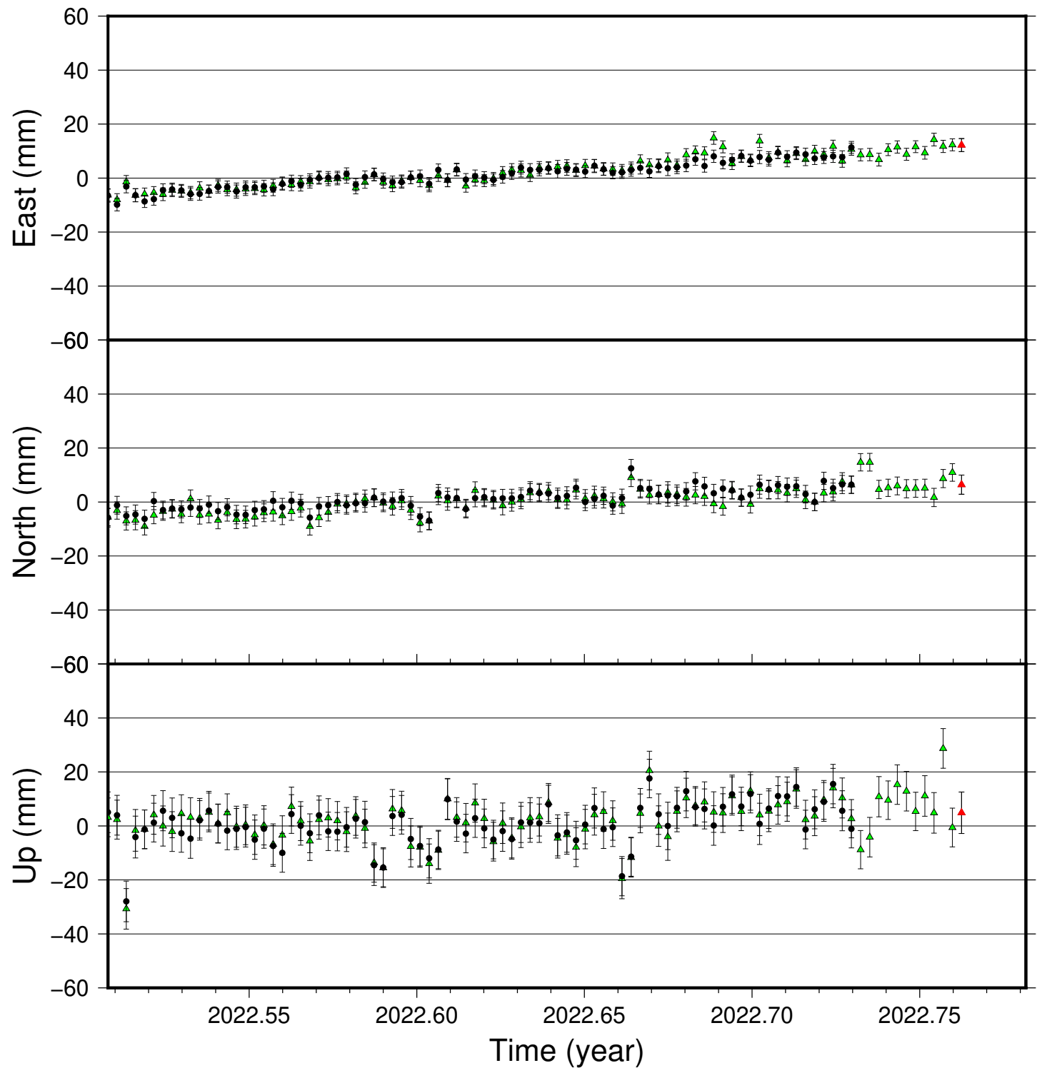
DYNG time series (IGS 2014), last 100 days
