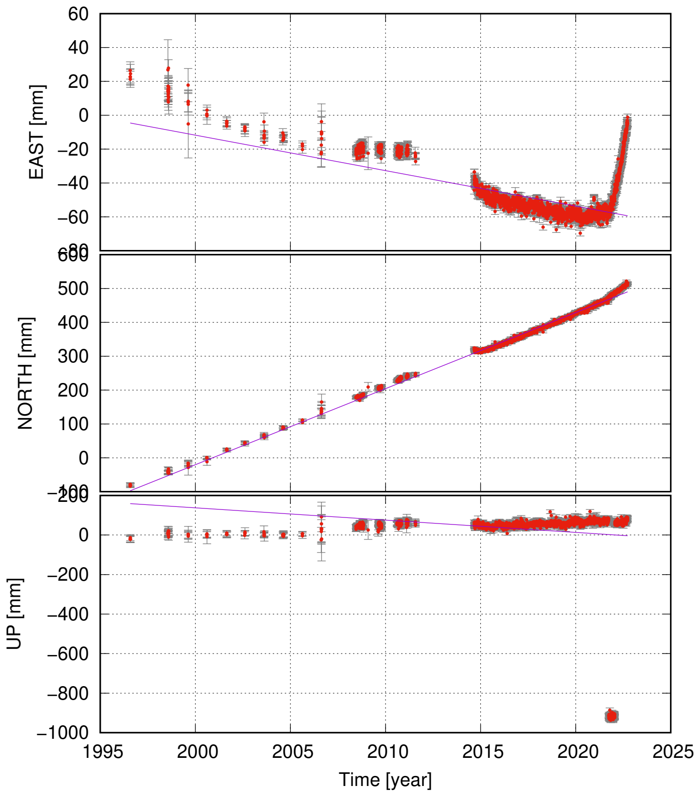
DYNG (65.06, -16.65) time series (ITRF 2014) v_e = -2.09 \pm 0.45 ; v_n = 22.45 \pm 0.30 ; v_u = -6.22 \pm 6.72 mm/yr
