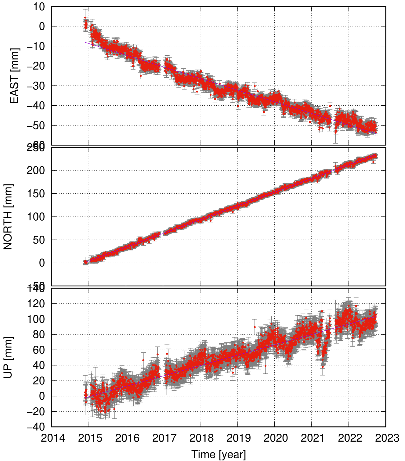
DYNY (65.02, -17.12) time series (ITRF 2014) v_e = -5.88 \pm 0.33 ; v_n = 29.74 \pm 0.30 ; v_u = 13.46 \pm 1.10 mm/yr
