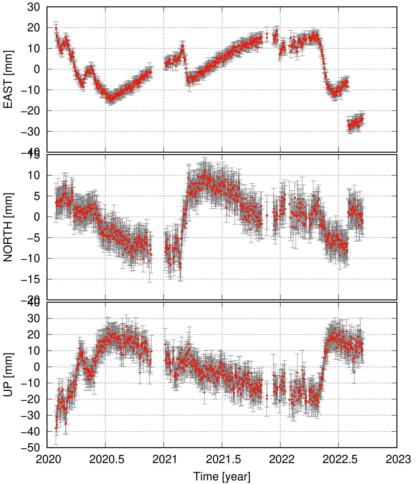
ELDC residual time series (some major events removed as well)
