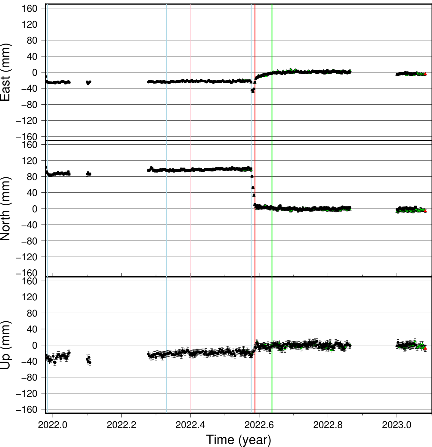
FAFC time series (IGS 2014), last 400 days
