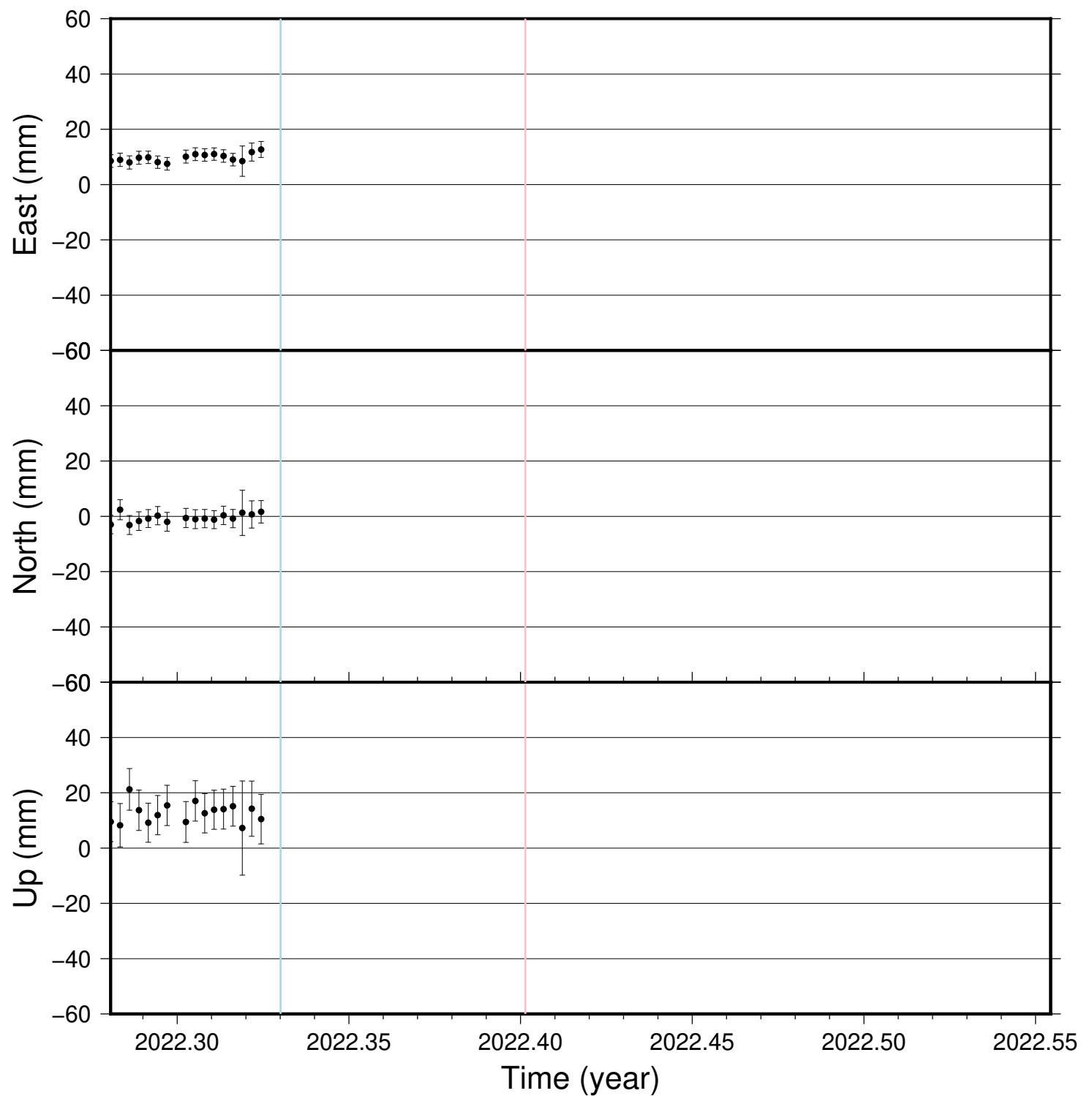
HAMD time series (IGS 2014), last 100 days
