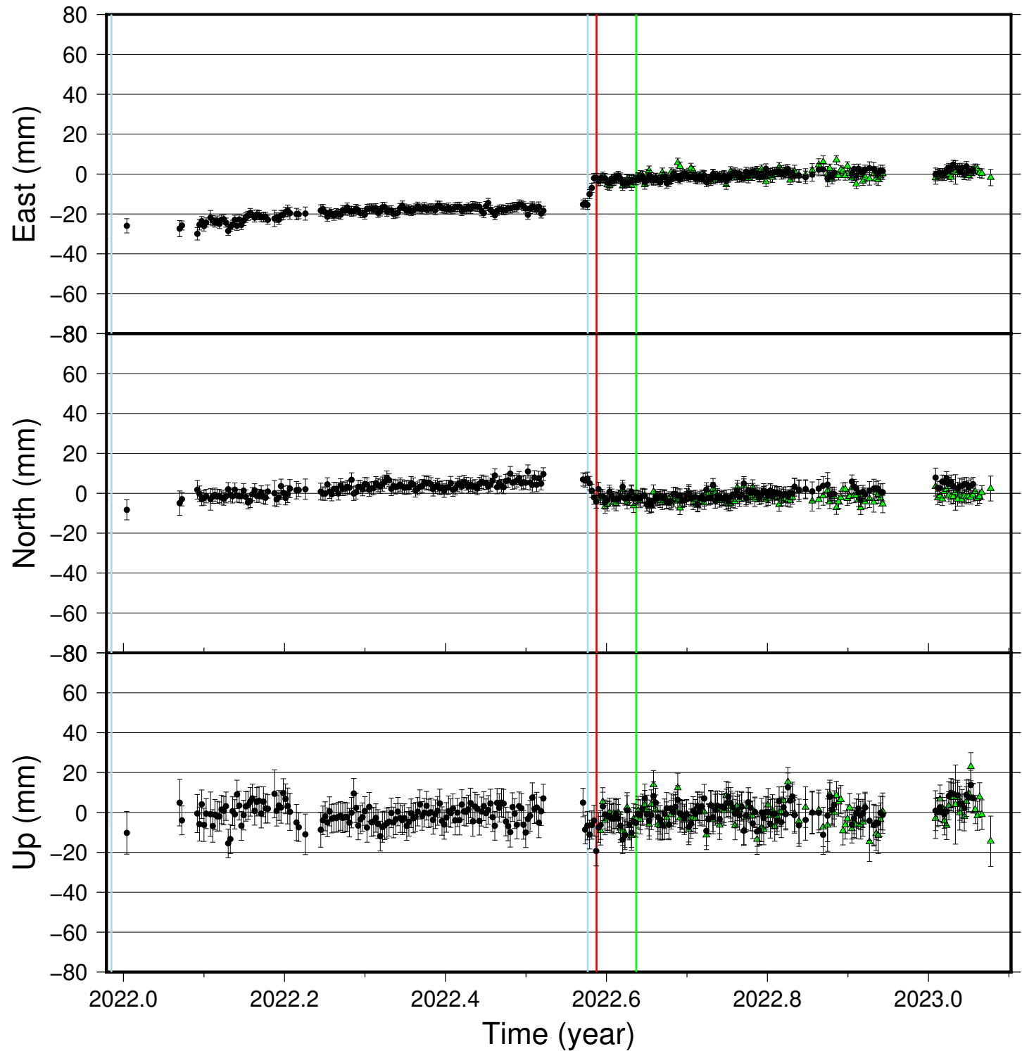
HERV time series (IGS 2014), last 400 days
