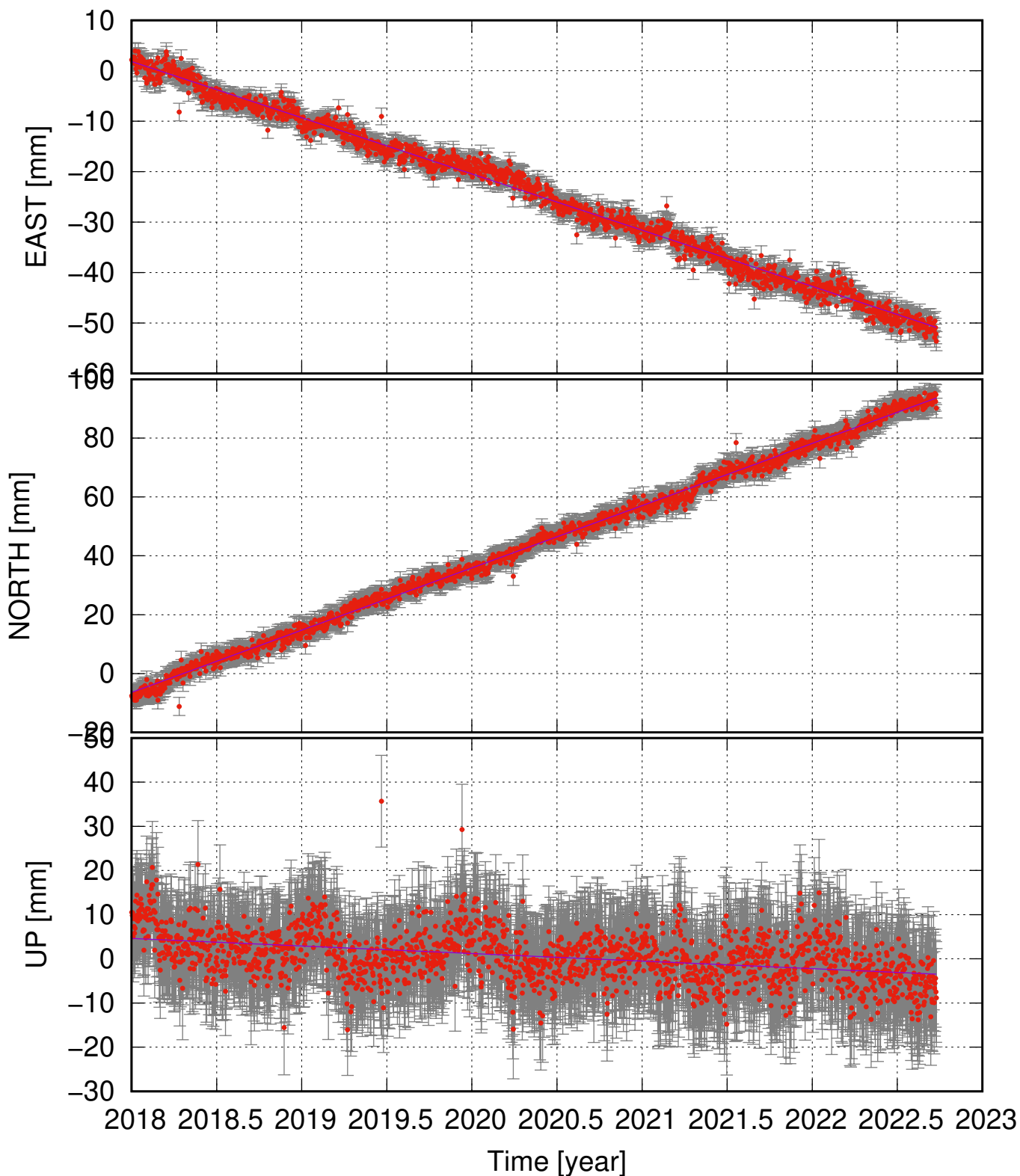
HRAC (66.11, -20.12) time series (ITRF 2014) v_e = -11.14 \pm 0.32 ; v_n = 21.15 \pm 0.36 ; v_u = -1.71 \pm 1.07 mm/yr
