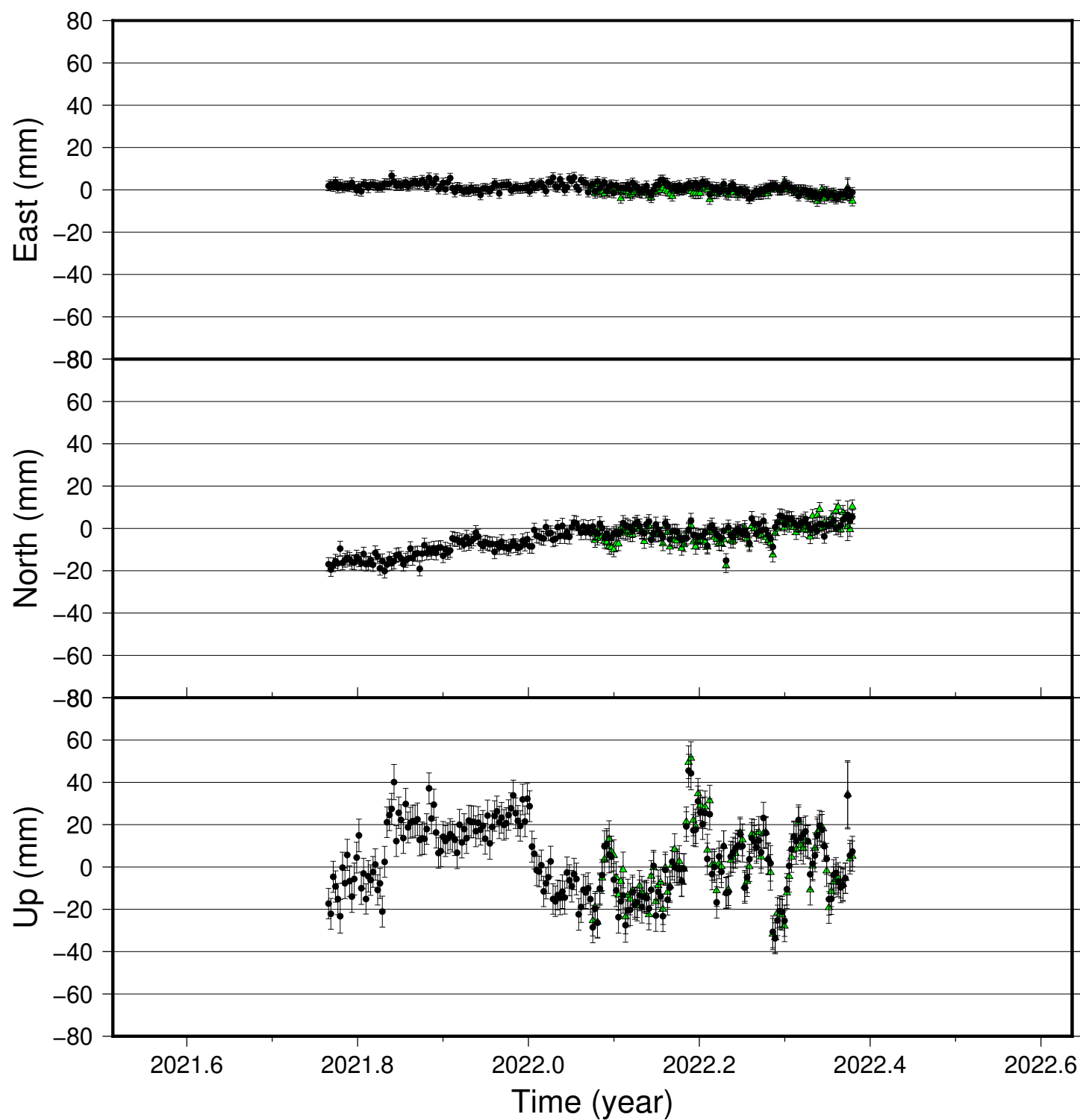
HRIC time series (IGS 2014), last 400 days
