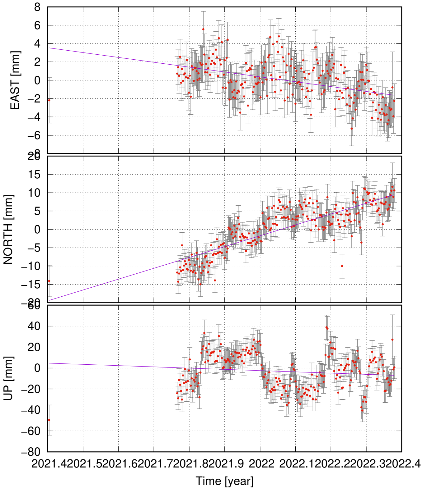
HRIC (64.95, -16.92) time series (ITRF 2014) ve = -5.30 \pm 1.88 ; vn = 29.58 \pm 3.63 ; vu = -11.94 \pm 17.24 mm/yr
