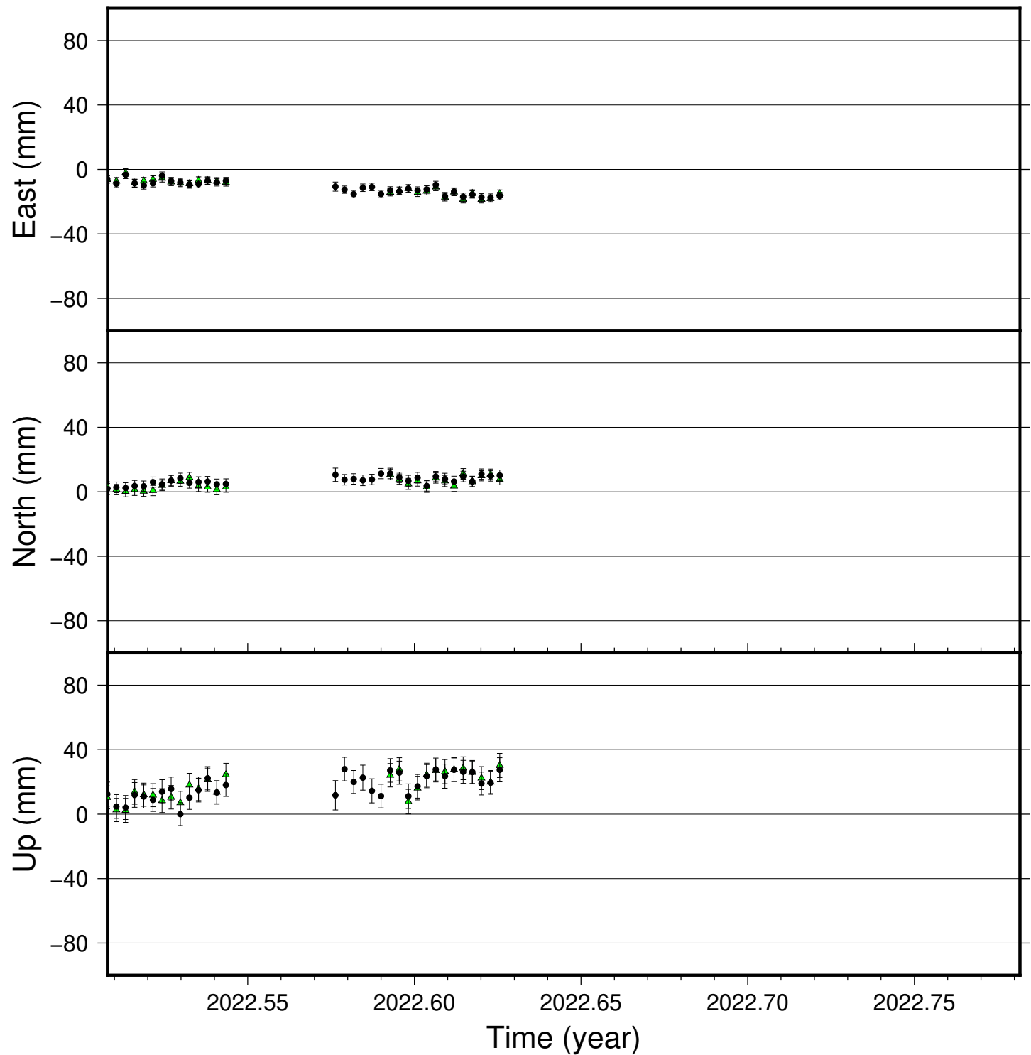
JONC time series (IGS 2014), last 100 days
