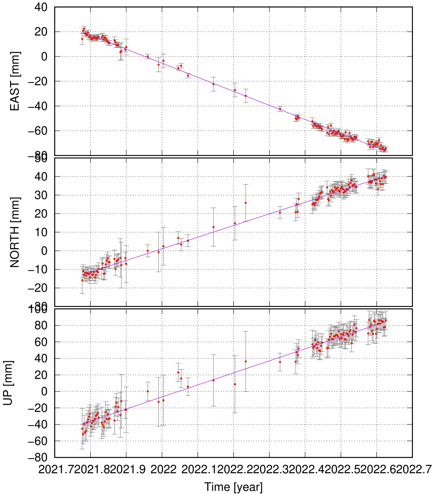
JONC (65.05, -16.83) time series (ITRF 2014) v_e = -113.54 \pm 2.52 ; v_n = 62.69 \pm 2.65 ; v_u = 145.86 \pm 7.59 mm/yr
