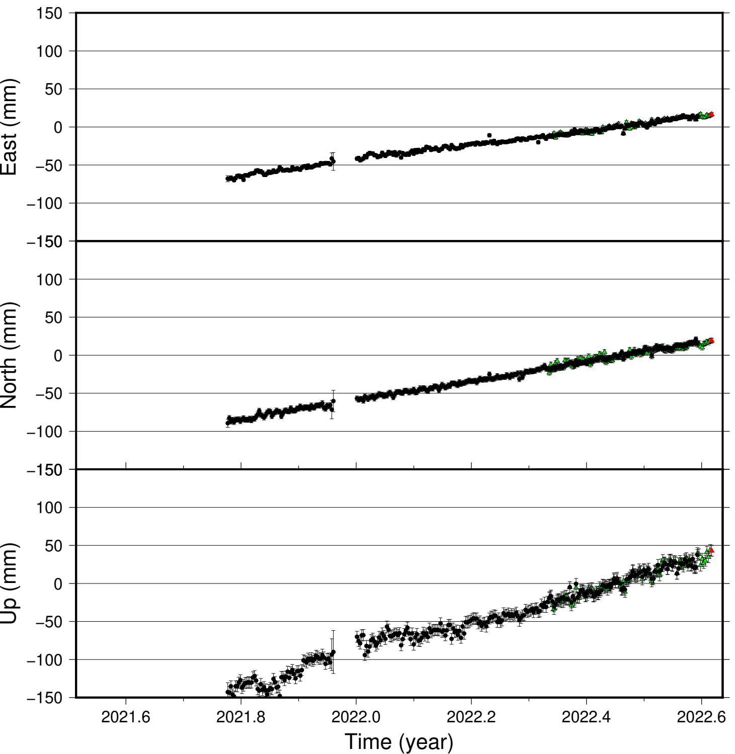
KASC time series (IGS 2014), last 400 days
