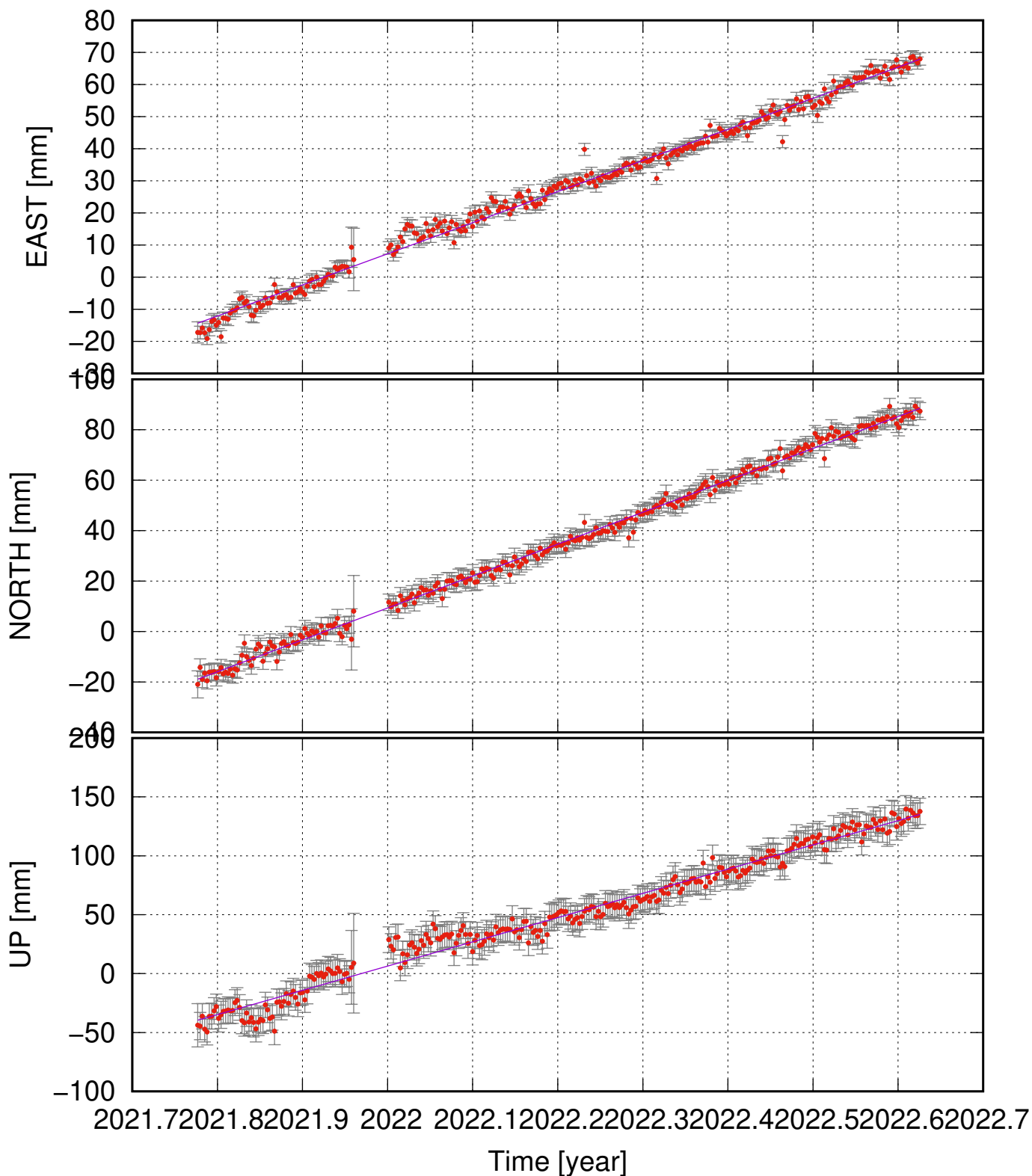
KASC (65.06, -16.76) time series (ITRF 2014) v_e = 96.89 \pm 2.65 ; v_n = 126.51 \pm 2.50 ; v_u = 205.81 \pm 9.09 mm/yr
