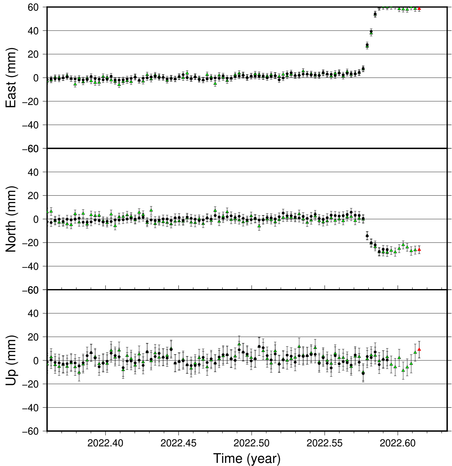
KRIV time series (IGS 2014), last 100 days
