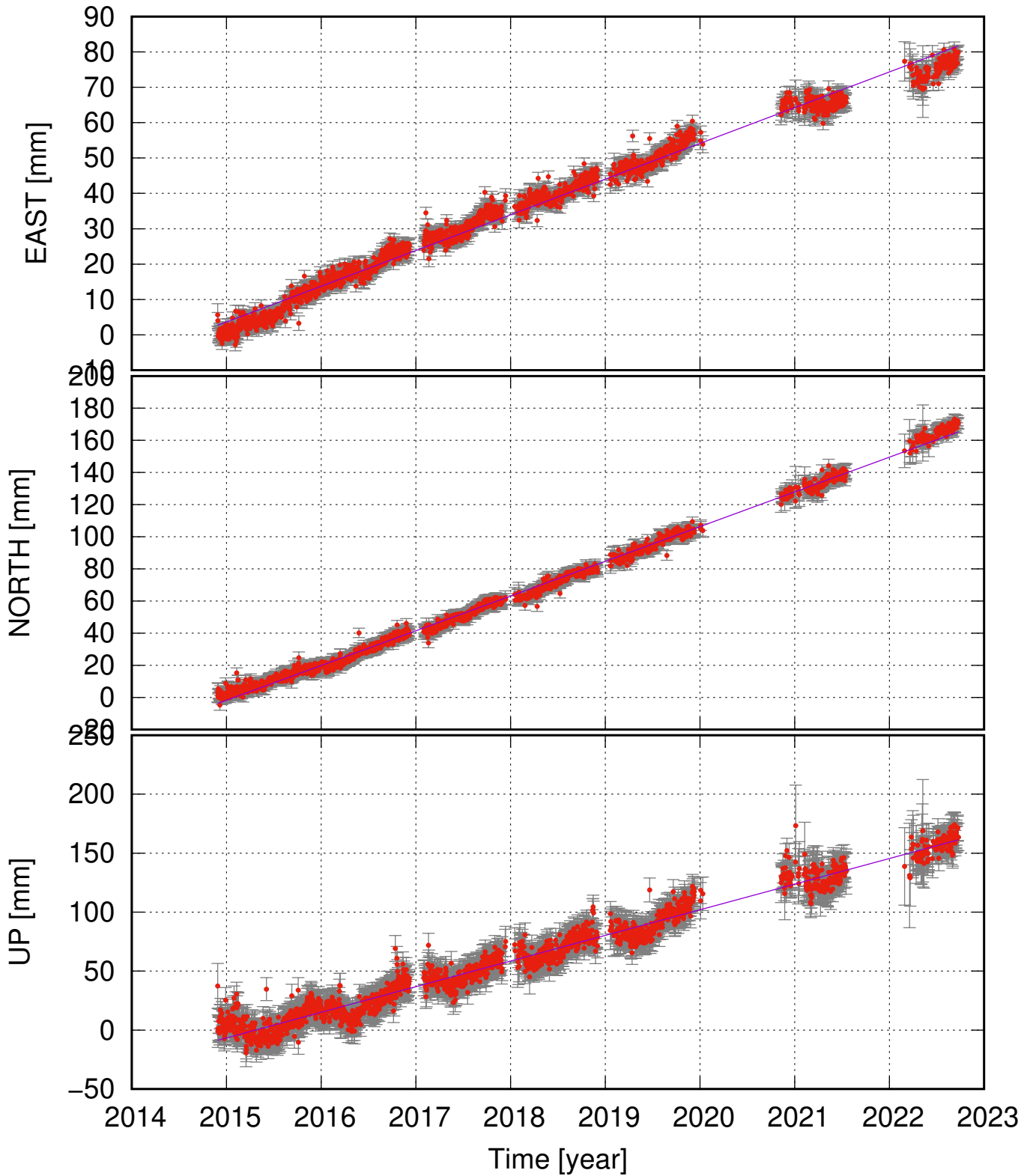
LANH (64.89, -16.56) time series (ITRF 2014) v_e = 10.10 \pm 0.32 ; v_n = 21.60 \pm 0.35 ; v_u = 21.74 \pm 1.06 mm/yr
