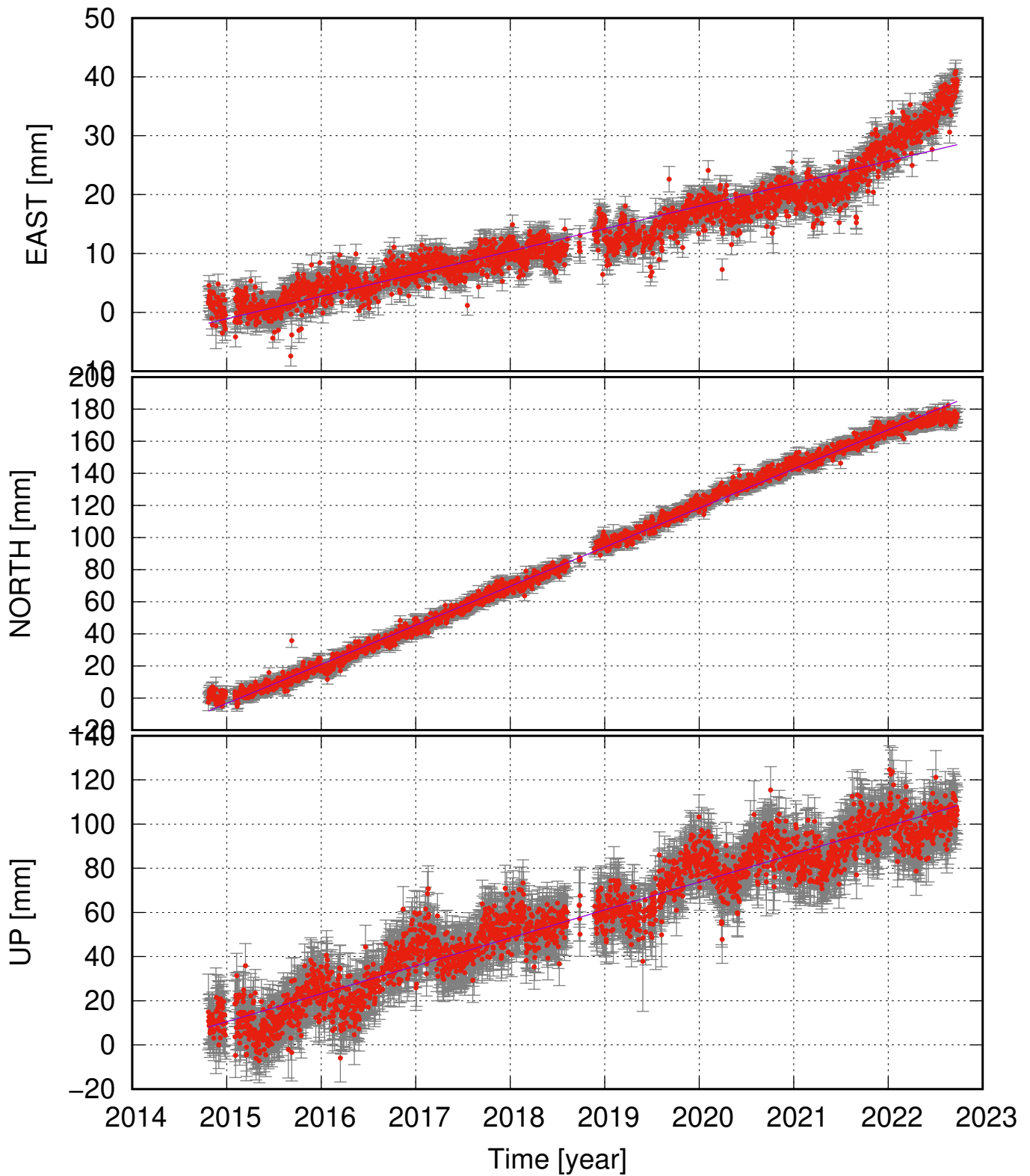
MOFC (64.98, -16.67) time series (ITRF 2014) v_e = 3.83 \pm 0.37 ; v_n = 24.34 \pm 0.43 ; v_u = 12.65 \pm 1.04 mm/yr
