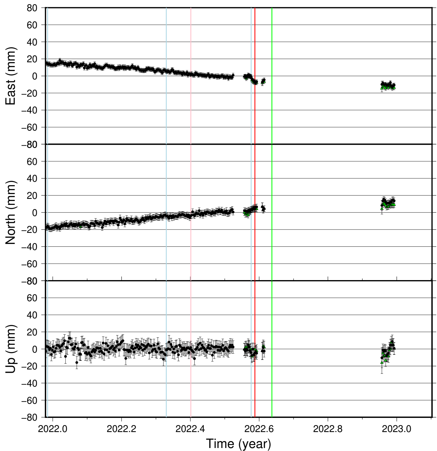
NYLA time series (IGS 2014), last 400 days
