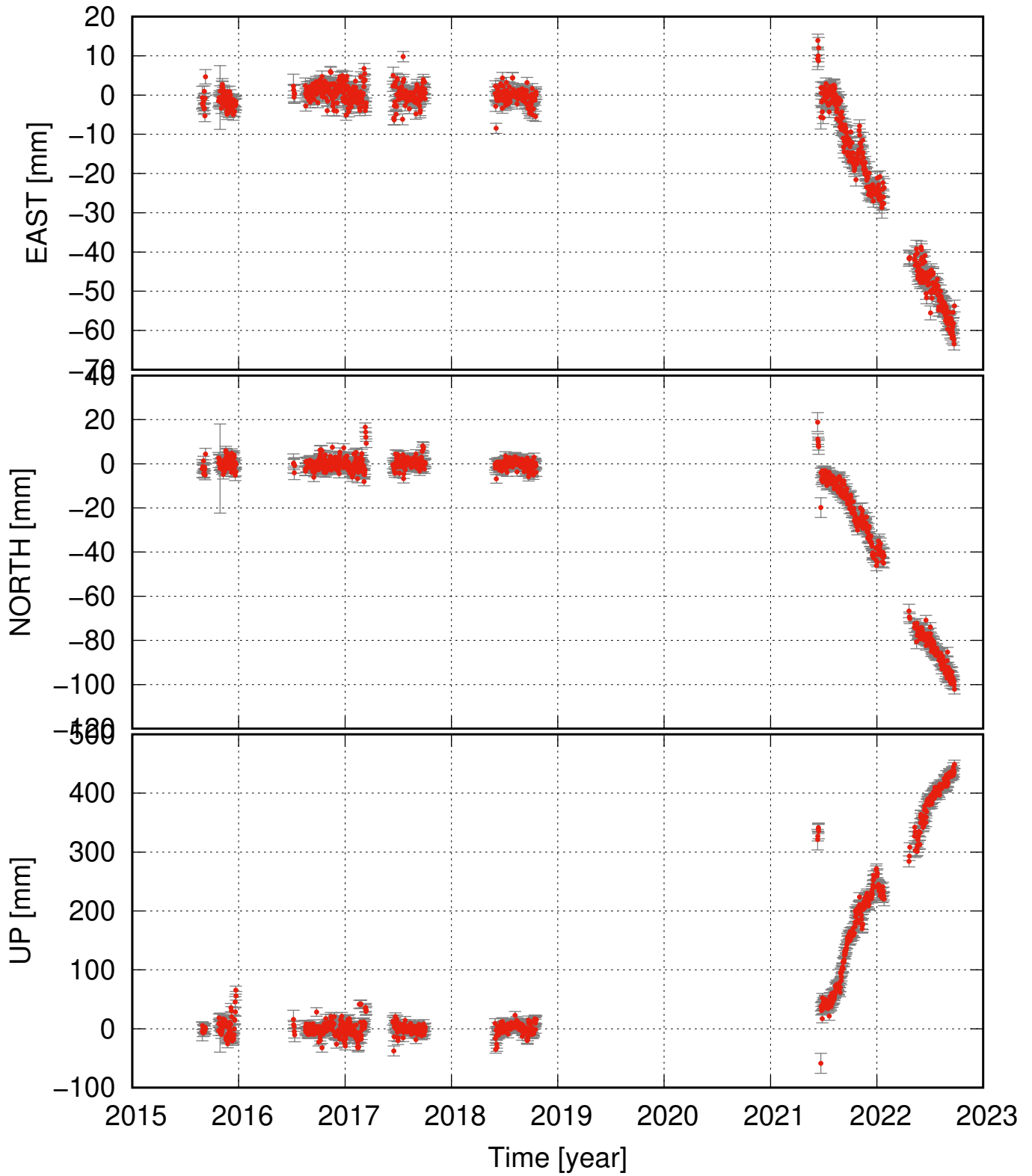
OLAC detrended and seasonal signal removed
