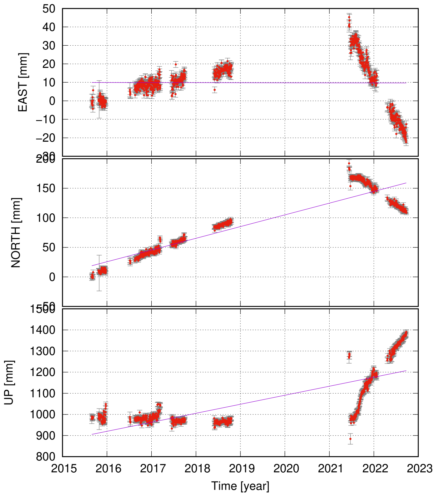
OLAC (65.04, -16.80) time series (ITRF 2014) ve = -0.04 \pm 1.74 ; vn = 19.81 \pm 2.82 ; vu = 42.71 \pm 11.67 mm/yr
