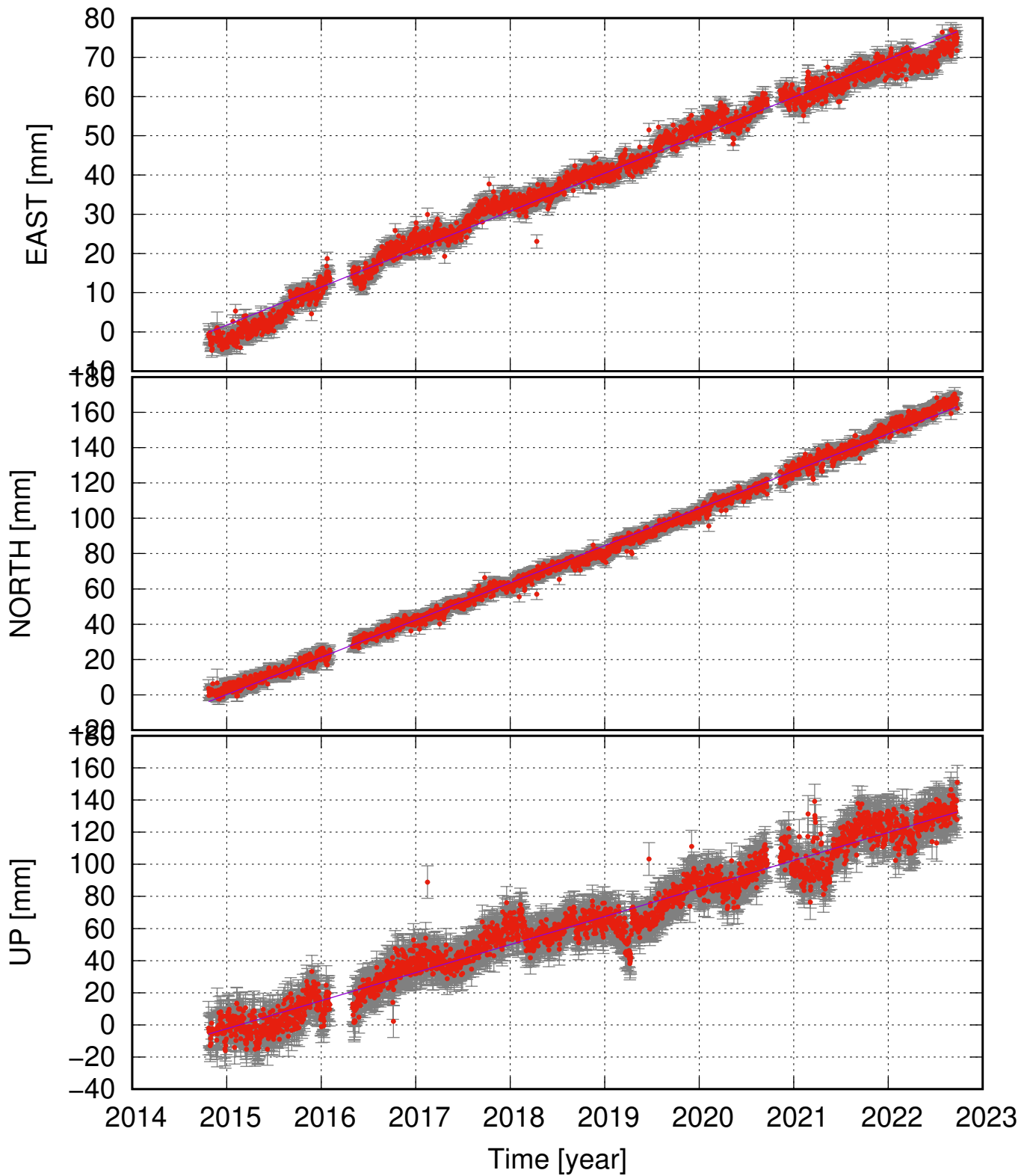
RIFC (64.92, -16.39) time series (ITRF 2014) v_e = 9.67 \pm 0.31 ; v_n = 21.08 \pm 0.35 ; v_u = 17.46 \pm 1.01 mm/yr
