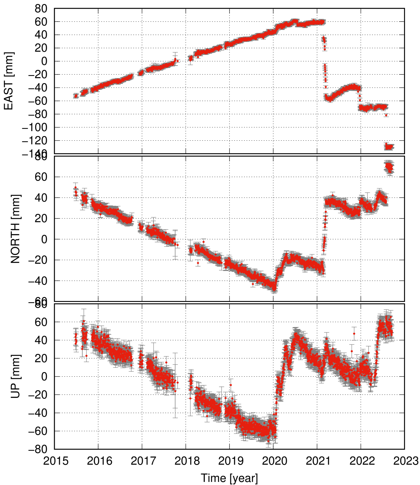
SENG residual time series (some major events removed as well)
