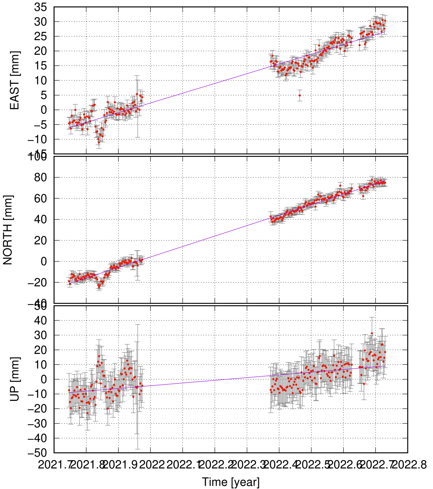
TANC (65.08, -16.74) time series (ITRF 2014) v_e = 33.14 \pm 2.67 ; v_n = 99.52 \pm 3.26 ; v_u = 18.41 \pm 7.66 mm/yr
