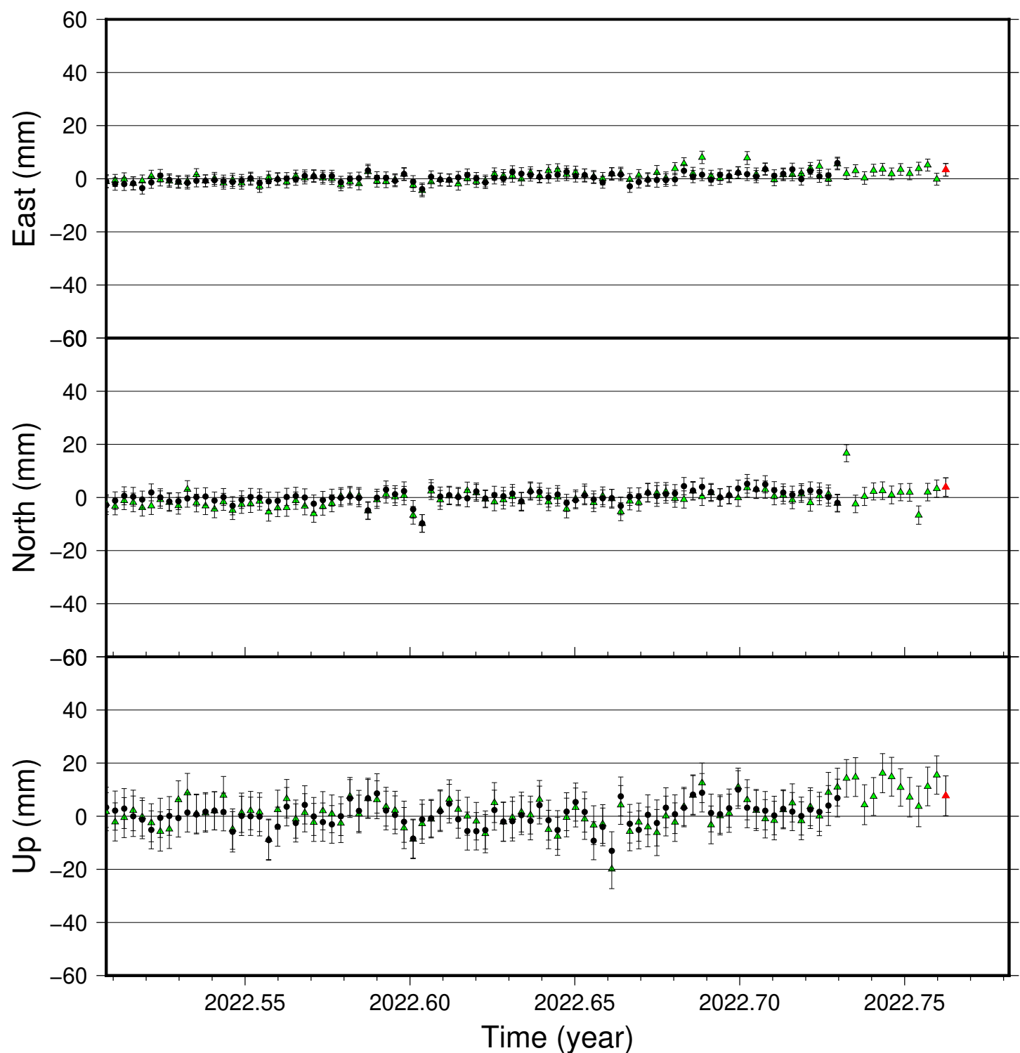
THOC time series (IGS 2014), last 100 days
