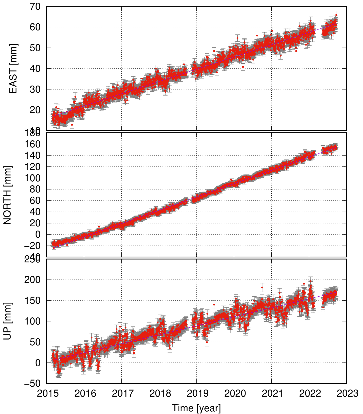
THOC (64.93, -16.68) time series (ITRF 2014) v_e = 5.92 \pm 0.25 ; v_n = 23.58 \pm 0.40 ; v_u = 21.68 \pm 1.74 mm/yr
