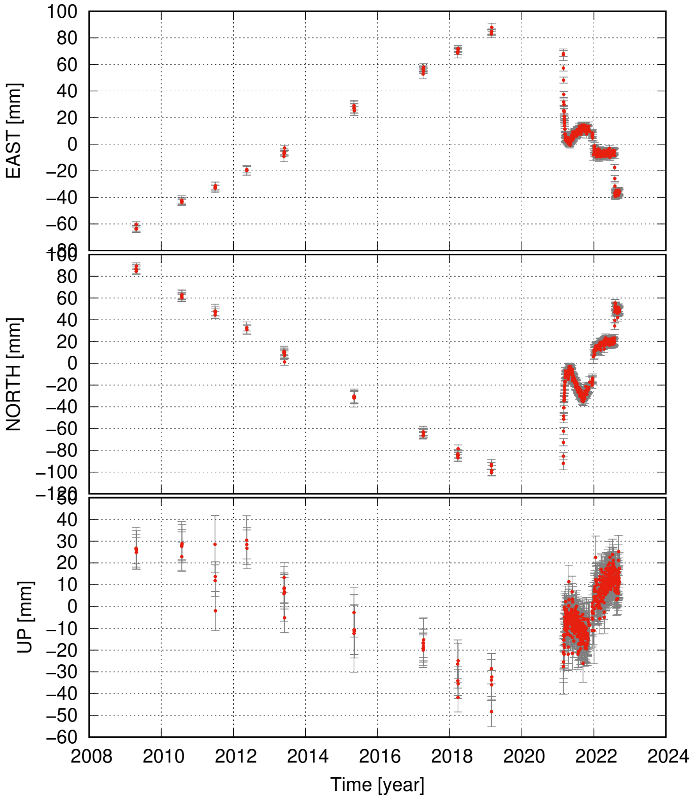
VOGC residual time series (some major events removed as well)
